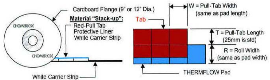
Figure 1 - T777 Material Structure
